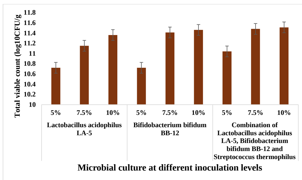
Fig. 1. Total viable count of probiotic cultures at different inoculation levels
