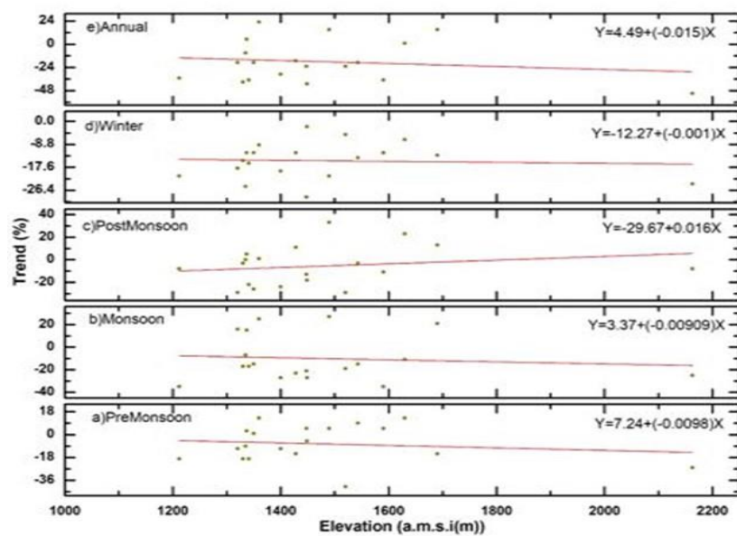
Fig. 6. Annual and seasonal Distribution of precipitation trends plotted against elevation
