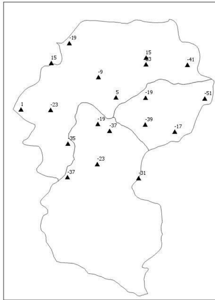
Fig. 5. Annual precipitation trend in Kathmandu Valley from 2003-2017
