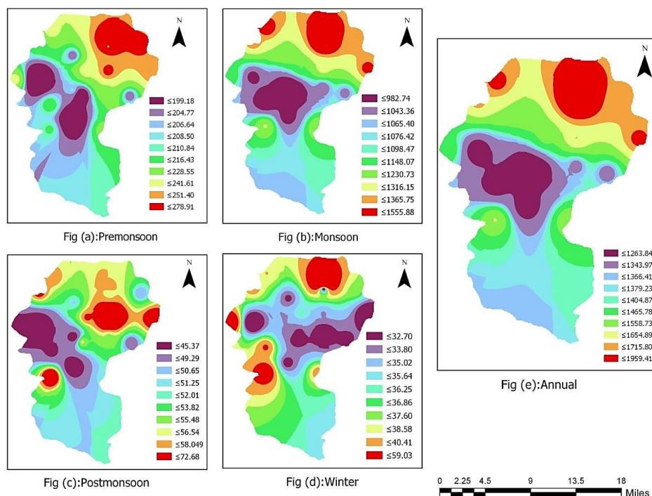
Fig. 1. Sesaonal and annual interpolation of rainfall using IDW tool
