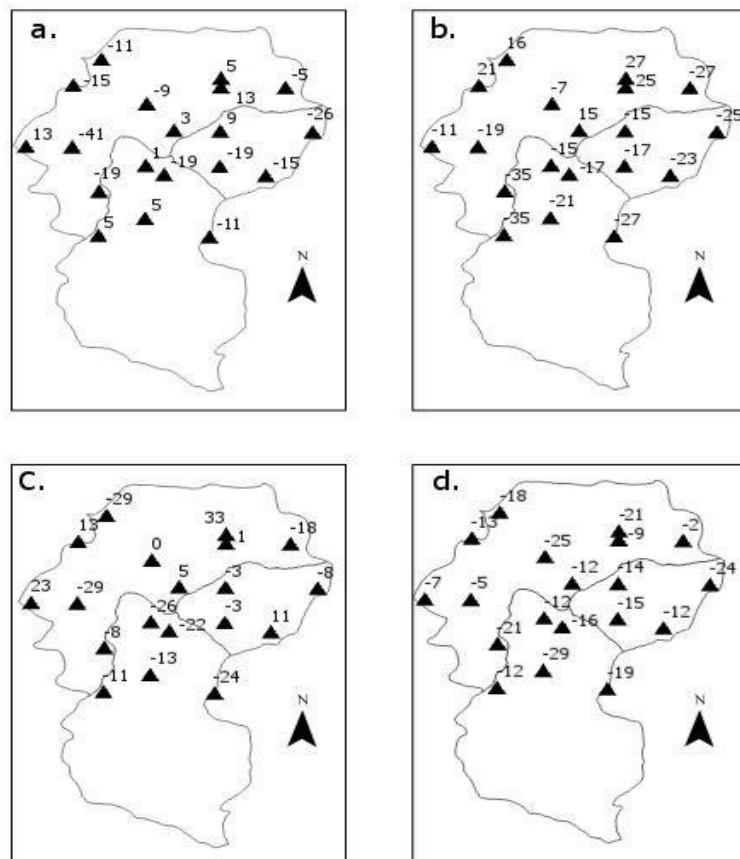
Fig. 4. Spatial Trend analysis of precipitation in a) Premonsoon b) Monsoon c) Postmonsoon d) Winter
