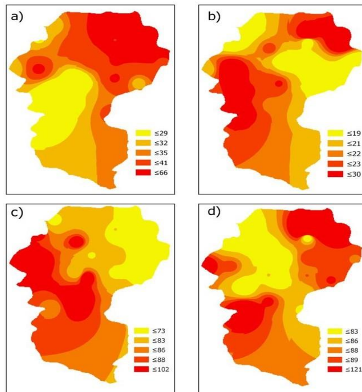
Fig. 3. Spatial Pattern of seasonal precipitation's CV's a) Pre-monsoon, b) Monsoon c) Post monsoon and d) Winter
