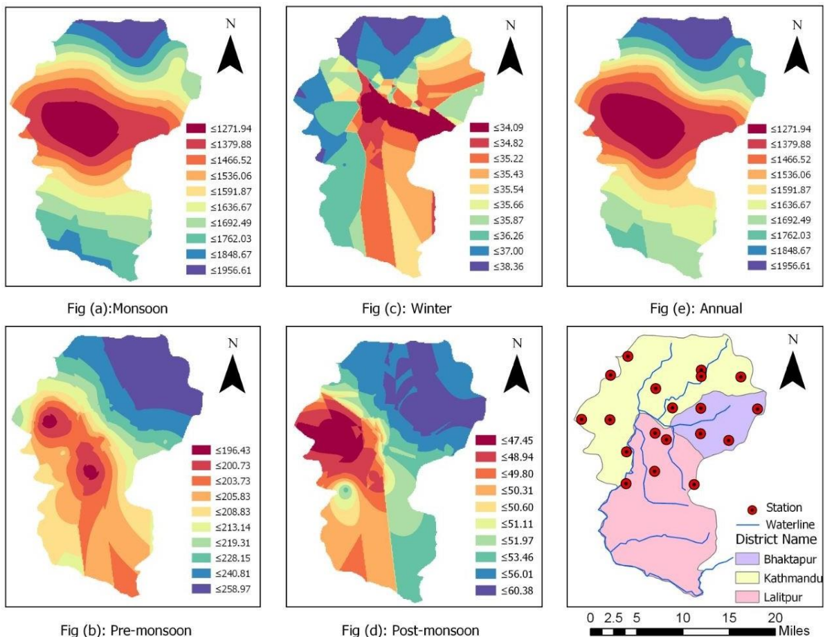
Fig. 2. Seasonal and annual Interpolation of rainfall using the Empirical Kriging Method
